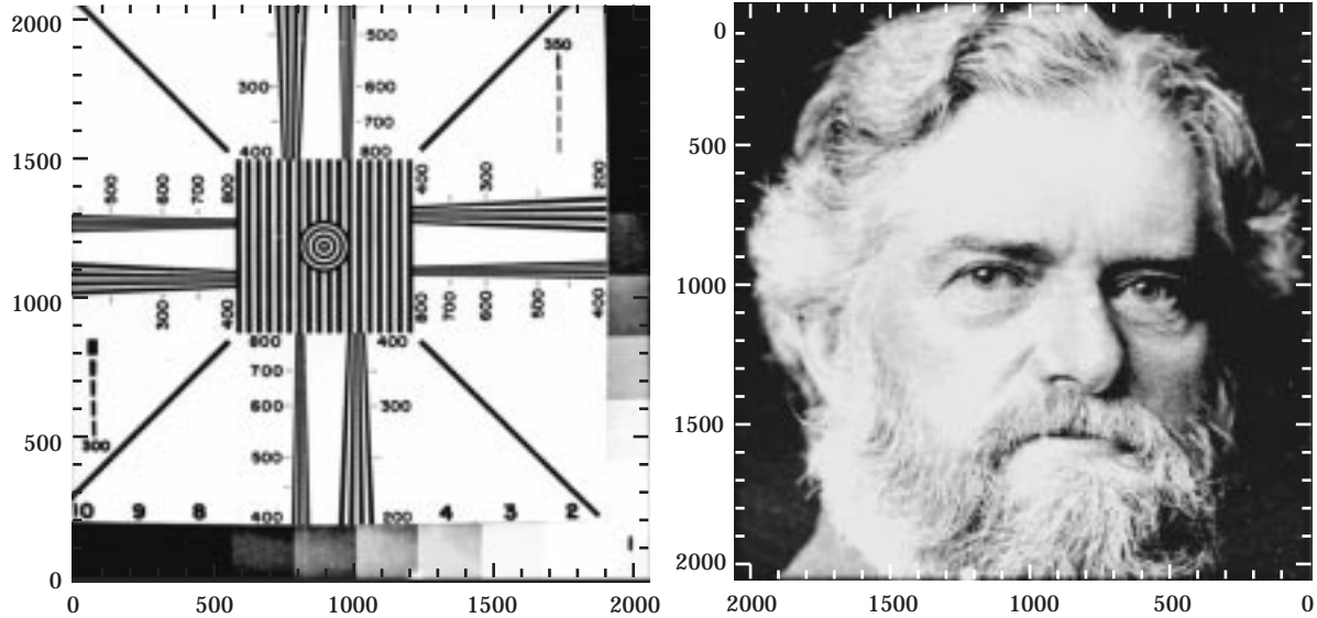
Fig. 7. Test image (of Simon Newcomb) taken with the first LBNL back-illuminated 2048 \times 2048 CCD.
