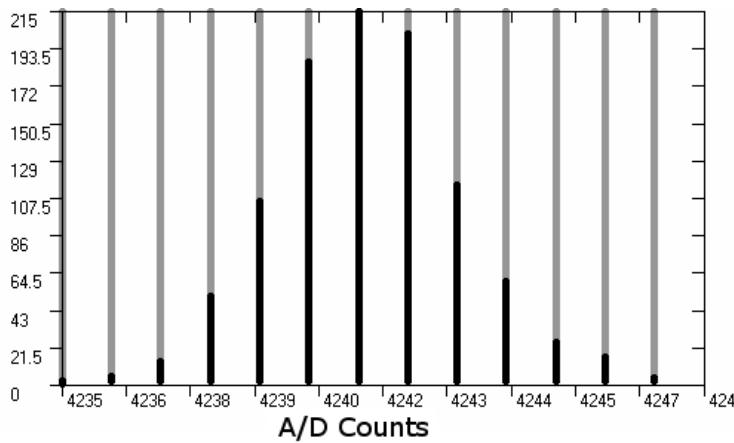
Figure 5. Noise histogram from 10000 samples at -110 C.
