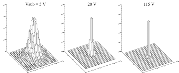
Fig. 2. The CCD response profile to a 1.2 \mu\text{m} rms beam spot for three different substrate bias voltages. Full depletion is reached at 20 V. Each grid box is a 10.5 \mu\text{m} pixel and the height is the detected charge.
