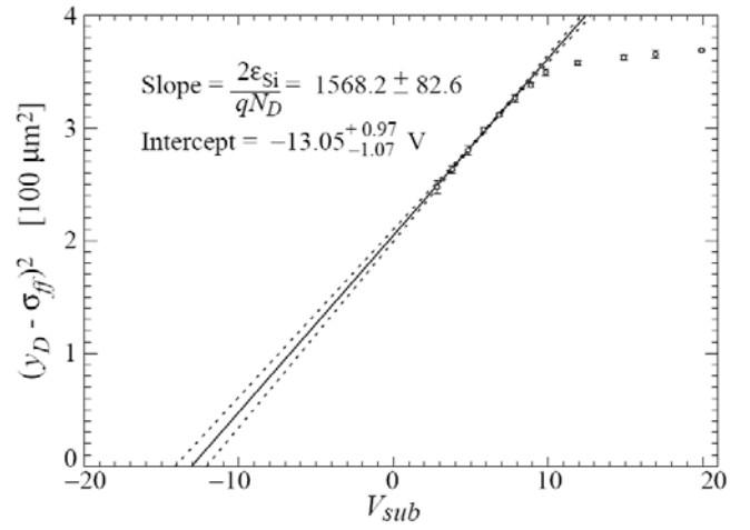
Fig. 5. The low-voltage linear fit used to determine parameters for the high-voltage fit. Here the square of the wafer thickness minus diffusion is plotted against the substrate voltage. The V_{sub} intercept is the junction voltage and the slope contains the carrier density.
