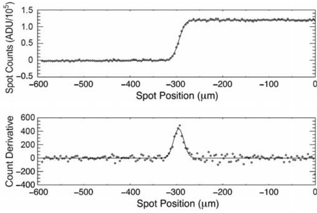
Fig. 3. Sample scan analysis. The top plot is the measured CCD counts in the integration area versus the beam position; the bottom plot is the derivative of the top. The top data can be fit with an error function, and the bottom data can be fit with a Gaussian. Both fits are obtained and compared as a consistency check. For these data, the error function sigma is 10.8 \pm 0.002 \mu\text{m} , and the Gaussian sigma is 10.9 \pm 0.6 \mu\text{m} .
