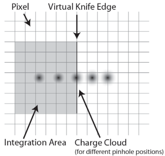
Fig. 1. The virtual knife edge concept. The spot is scanned to the right over the pixels on the CCD and eventually exits the integration area. The summed charge in the area square exhibits an error function shape.
