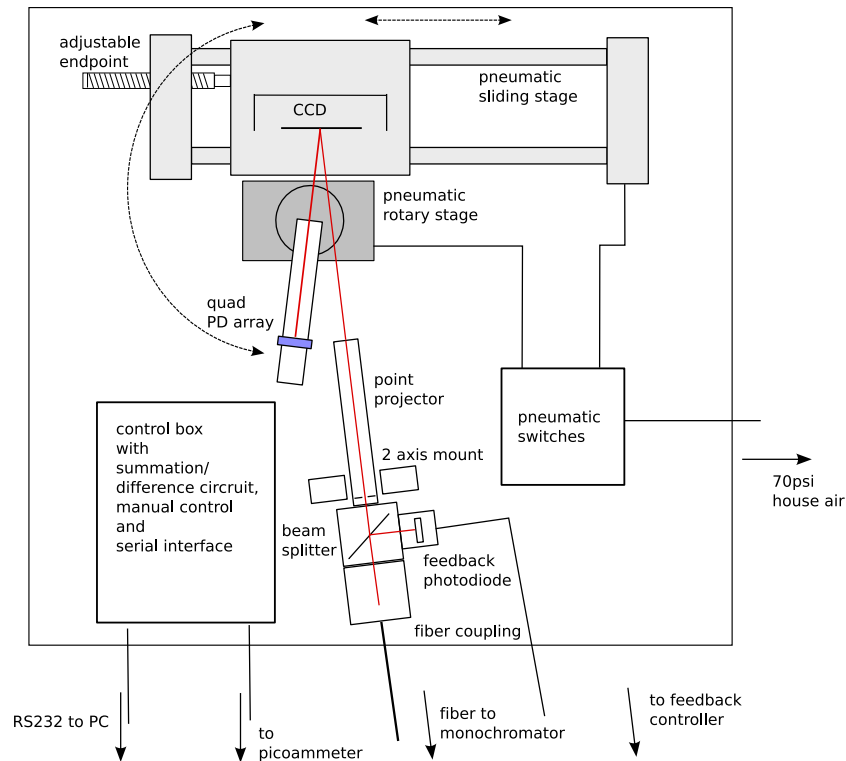
Figure 5. The reflectometer. The CCD is mounted on a pneumatic sliding stage. It can be adjusted for tilt around two axis and for focus. A point projector equipped with a feedback assembly for light stabilization provides the probing beam. A quad-array photodiode measures first the light beam directly then the reflected beam. Using a quad array allows careful beam centering.
