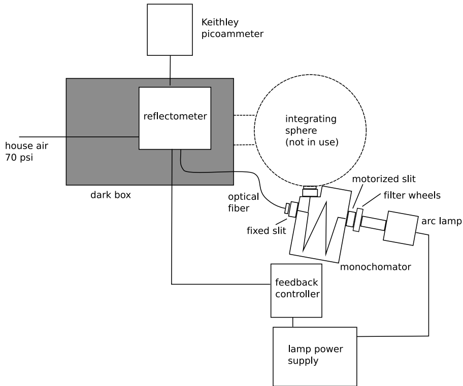
Figure 4. The reflectometer setup. The lightsource, monochromator and dark box are the same as in the QE setup. The reflectometer resides in the dark box.
