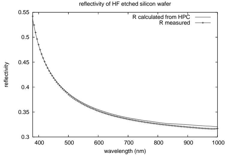
Figure 7. Shows the measured reflectivity of a piece of a silicon wafer and the calculated reflectivity. The wafer was HF etched before the measurement to eliminate surface contamination. The measured and the calculated curve show good agreement. The absolute difference is not larger than 0.005.
