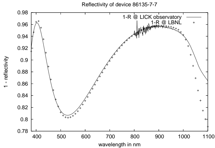
Figure 8. 1 - R for device 86135-7-7 measured at LBNL and the UCO/Lick observatory.
