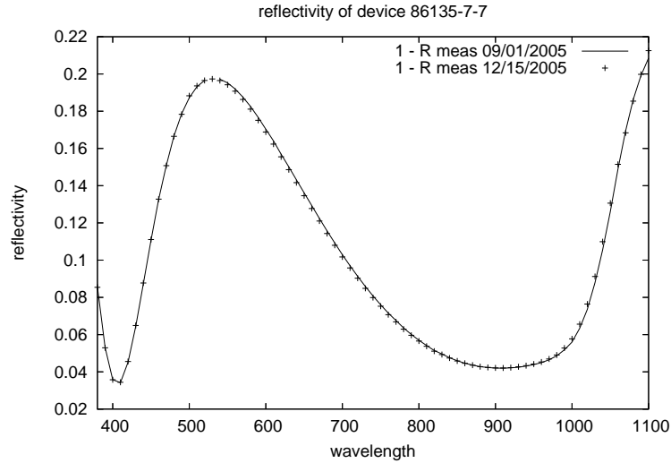
Figure 9. The two measurements of 1 - R for device 86135-7-7 match well.
