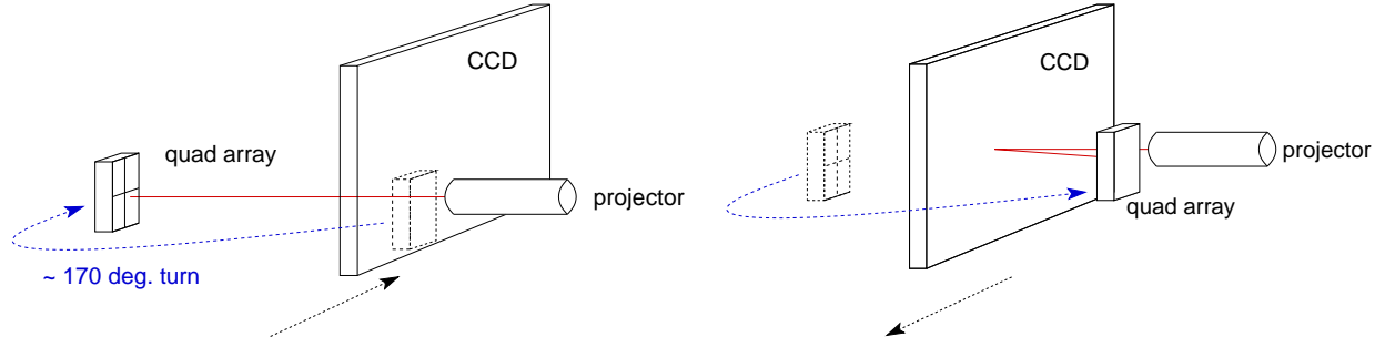
Figure 3. Left: The CCD is moved out of the optical path of the projector and the photodiode is moved in. The cumulative photocurrent gives I_0 .
