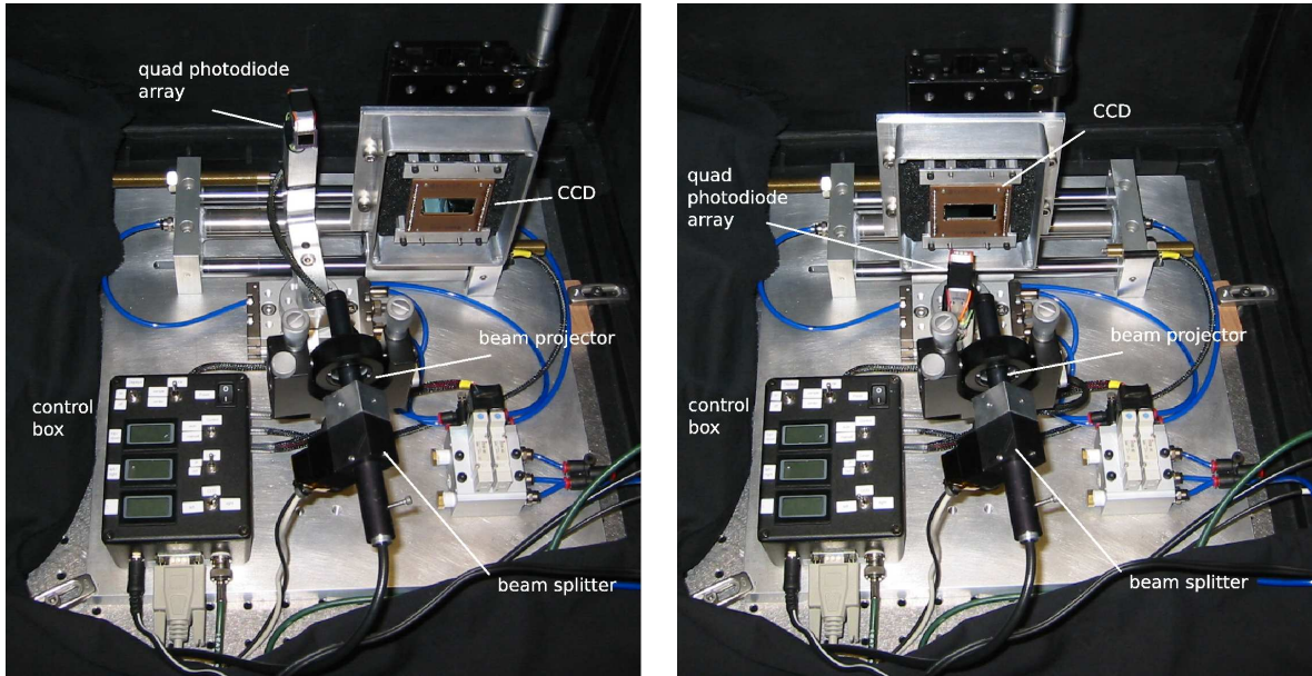
Figure 6. The actual reflectometer. A CCD is mounted to be tested.
