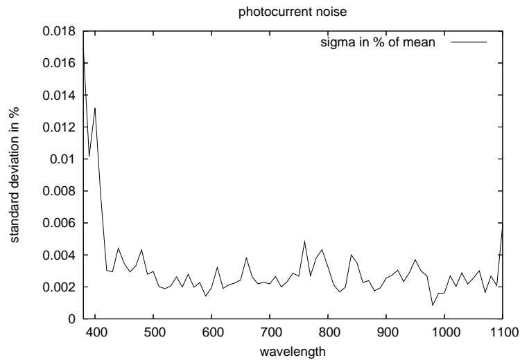
Figure 10. Shows the noise of I_{\text{ref}} from one scan.
