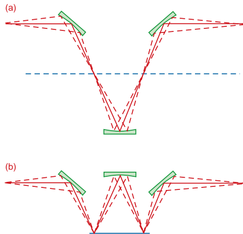
Figure 2. The VW scheme. a) First the monochromatic light beam is reflected off three mirrors giving the reference signal. b) Then the sample, here the CCD, is moved between the mirrors and one mirror is moved to the other side of the probe to give the reflected signal. The ratio of the both signals gives R^2 .
